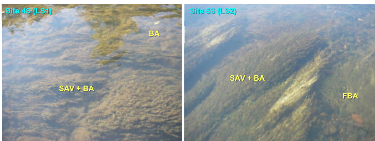
Figure 4. Examples of the common occurrence of abundant benthic algae in (BA), including filamentous forms (FBA), in locations where submersed aquatic vegetation (SAV) covered 20% or more of the area. Photos of Sites LS1 and LS2 (Hafele 2013) correspond to Stillwater Sciences (2020) Sites 4S and 5S.
