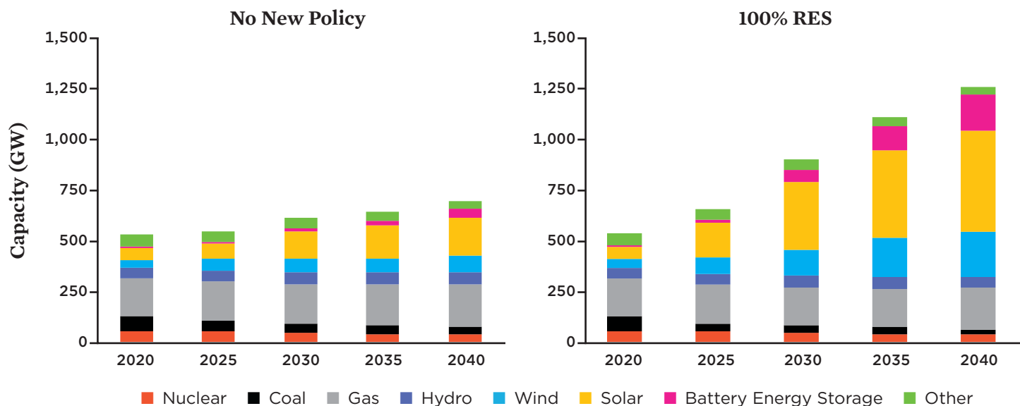
FIGURE 3. Electricity Capacity in USCA States in Two Scenarios, 2020–2040
